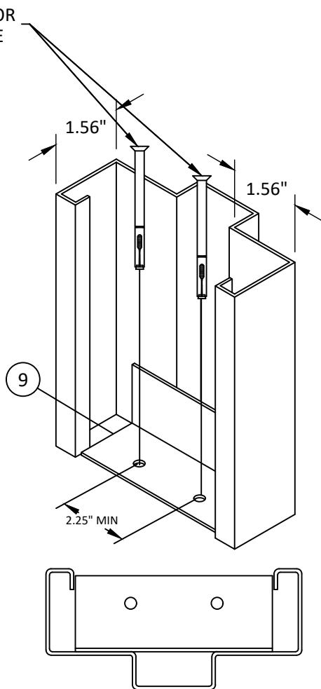
DETAIL BB WELDED BASE ANCHOR
